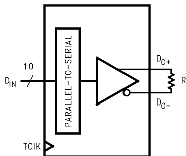
Figure 11. Serializer Delay
