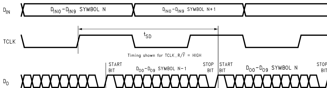
Figure 11. Serializer Delay
