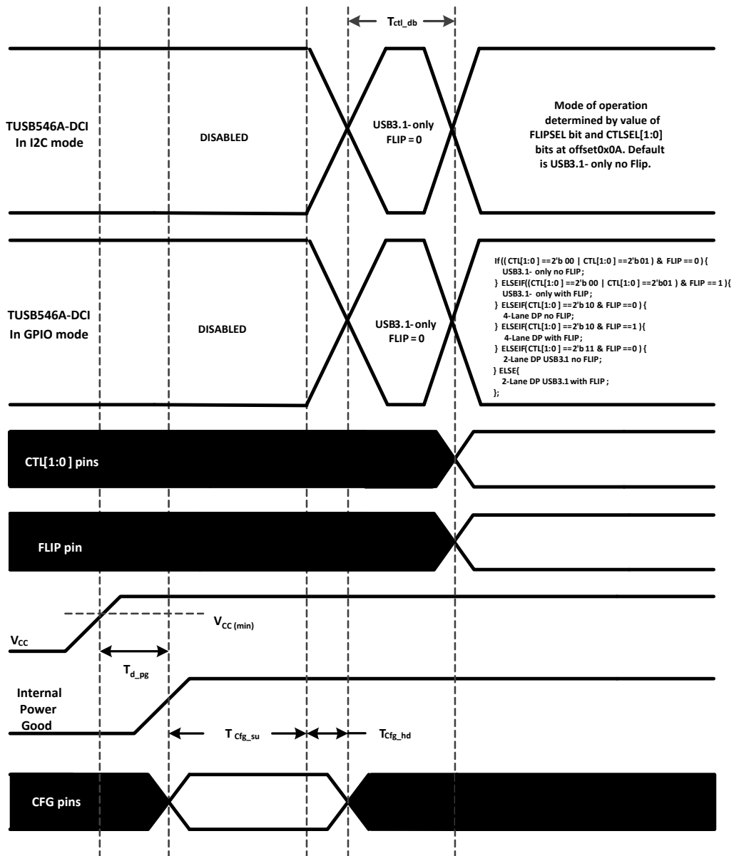
Figure 18. Power-Up Timing
