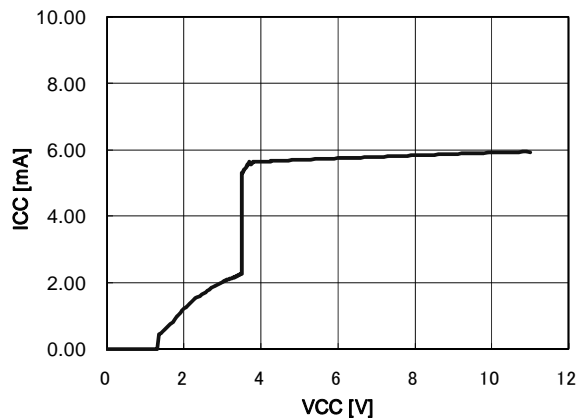
Fig. 11 Circuit current vs supply voltage (all cannels ON)
