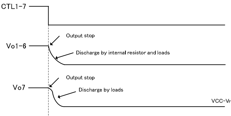
Fig. 6 stop sequence
