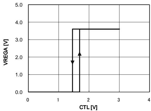
Fig. 20 CTL terminal characteristic
