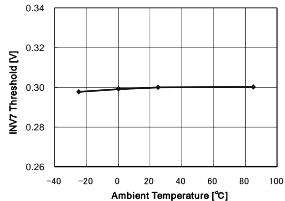
Fig. 17 CH7 ErrorAmp. INV threshold vs ambient temperature
