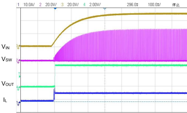
(19) Power Ramp Up (VIN=50.0V, VOUT=3.3V, IOUT=0.6A)
