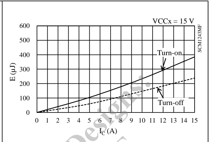
Figure 15-49 Low-side Switching Loss ( T_j = 25\text{ }^\circ\text{C} )
