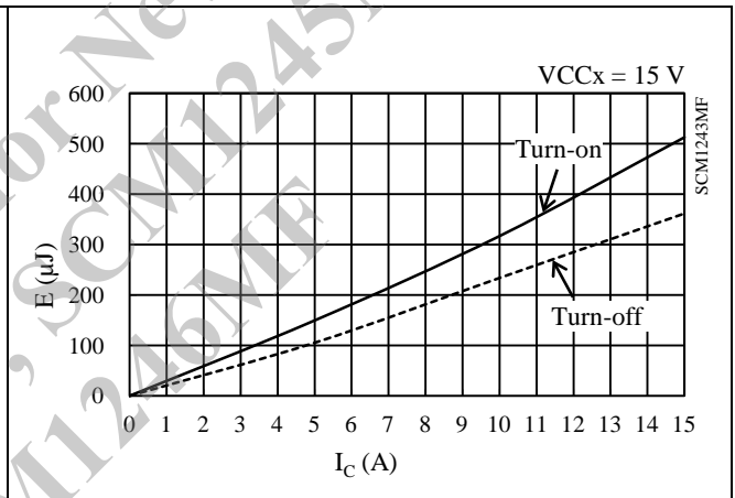
Figure 15-51 Low-side Switching Loss ( T_j = 125\text{ }^\circ\text{C} )
