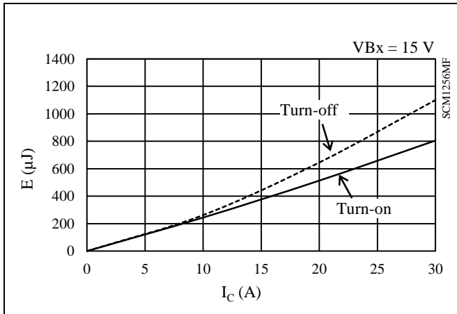
Figure 15-60. High-side Switching Loss ( T_j = 25^\circ\text{C} )
