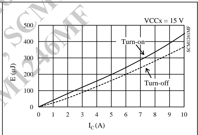
Figure 15-39. Low-side Switching Loss ( T_j = 125^\circ\text{C} )
