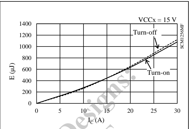
Figure 15-61. Low-side Switching Loss ( T_j = 25^\circ\text{C} )
