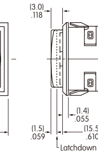
Single Color LED Side View
