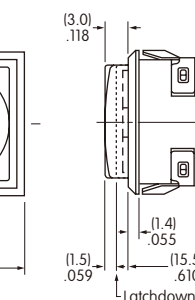
Bicolor LED Side View
