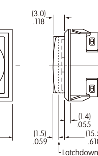
Single Color LED Side View
