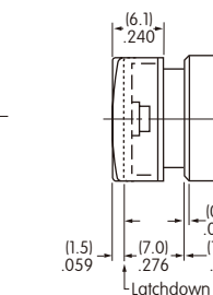
Bicolor LED Side View
