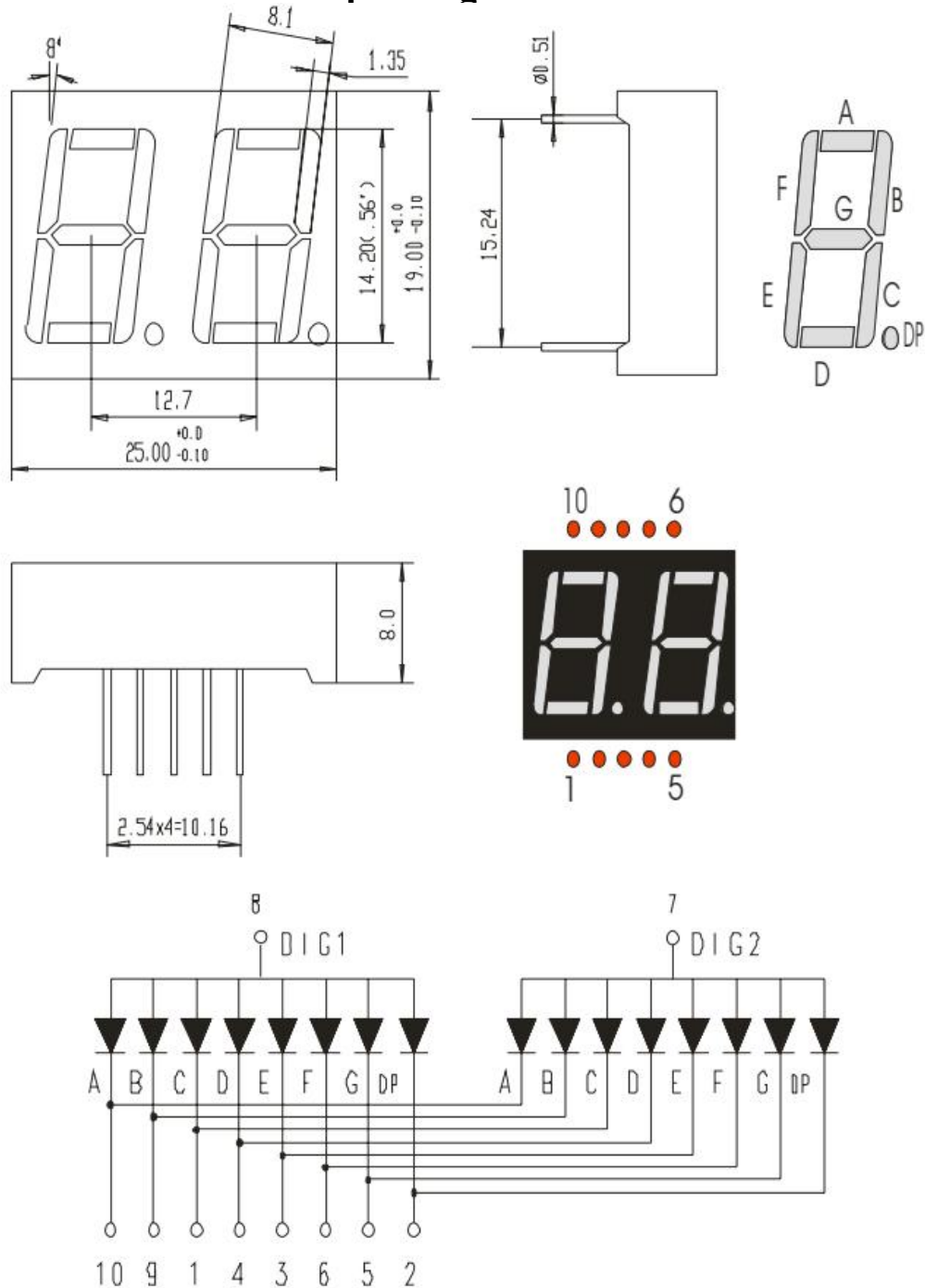
Figure Size & Circuit Principle Diagram : 25mm×19mm×8.0mm
