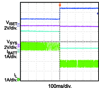
Charge Off
