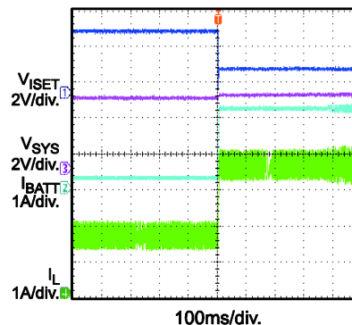
Charge On
