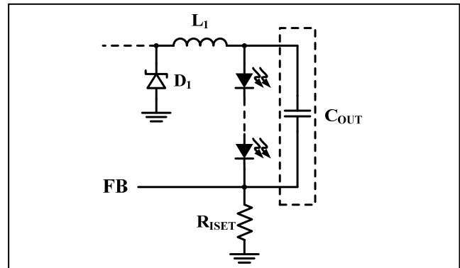
Figure 29 Adding Output Capacitor
