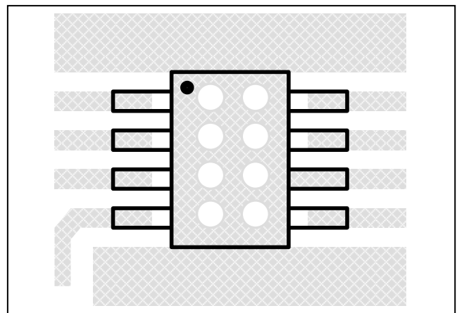
Figure 36 Board Via Layout For Thermal Dissipation
