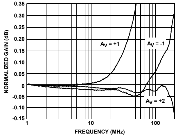
FIGURE 18. GAIN FLATNESS
