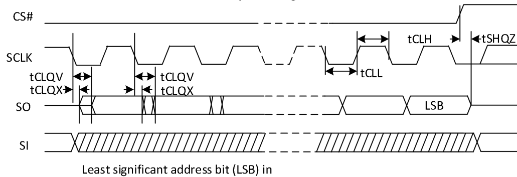
Output Timing
