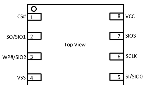
Figure1. Connection Diagram
