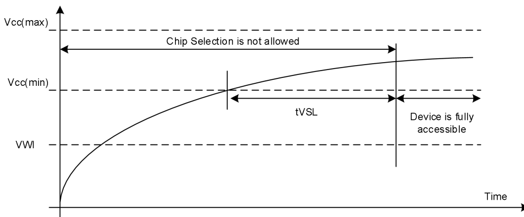
Figure26. Power-On Timing
