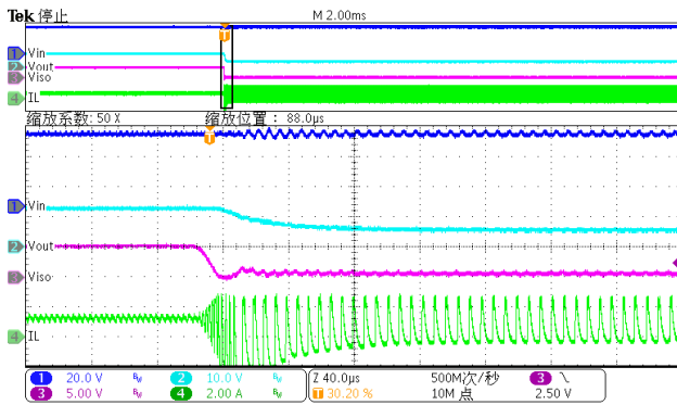
Figure 29. Secondary-Side Short(Io=1.2A)
