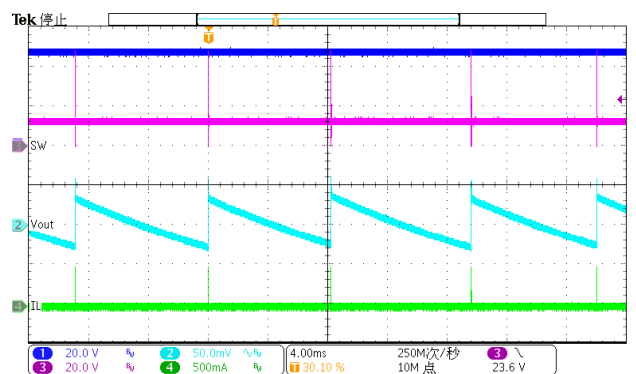
Figure 21. Output Ripple (Iload=0A, PFM)
