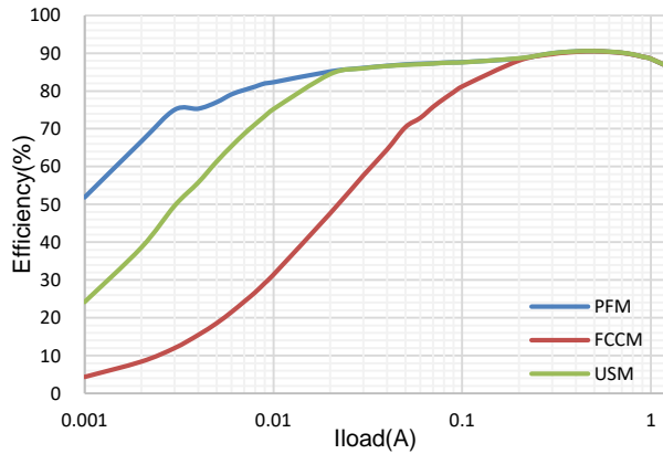
Figure 2. Efficiency, Vin=48V, Vout=12V
