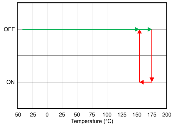
Figure 6-32. Thermal Shutdown
