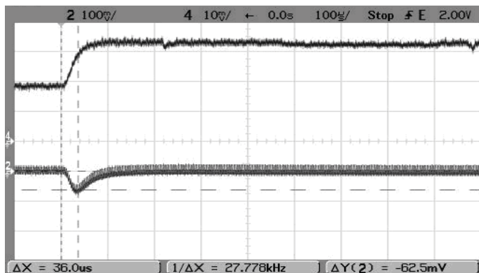
Step Load Transient Response (Vin=5V, Vout=1.8V, Cload=0, Iout=1.5A to 3A) Trace 2=Vout, 100 mV/div. Trace 4=Iout, 1A/div.
