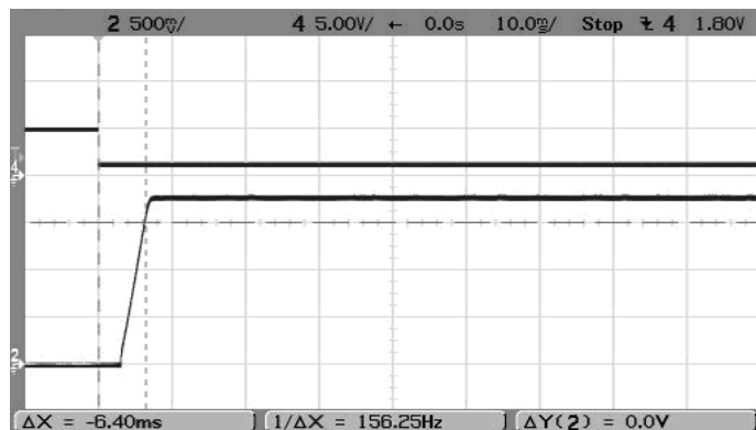
On/Off Enable Startup (Vin=5.5V, Vout=1.8V, Iout=5A, Cload=0)
