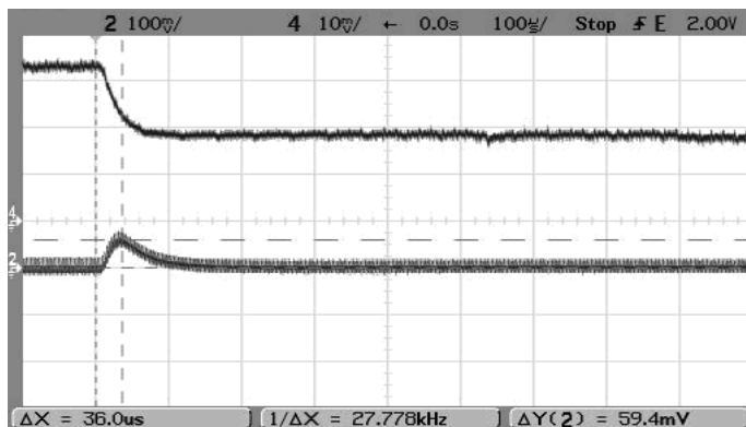
Step Load Transient Response (Vin=5V, Vout=1.8V, Cload=0, Iout=3A to 1.5A) Trace 2=Vout, 100 mV/div. Trace 4=Iout, 1A/div.
