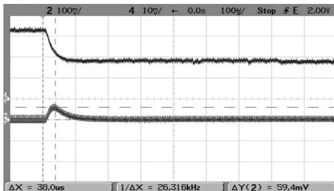
Step Load Transient Response (Vin=5V, Vout=1.2V, Cload=0, Iout=3A to 1.5A)
