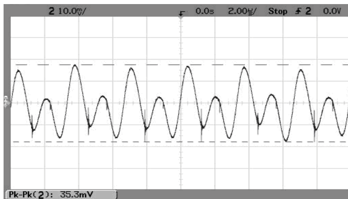
Output Ripple and Noise (Vin=5V, Vout=1.5V, Iout=5A, Cload=0, ScopeBW=100MHz)
