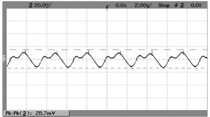
Output Ripple and Noise (Vin=5V, Vout=2.5V, Iout=3A, Cload=0, ScopeBW=100MHz)
