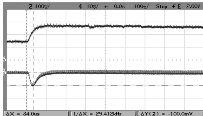
Step Load Transient Response (Vin=5V, Vout=1.8V, Cload=0, Iout=2.5A to 5A)
