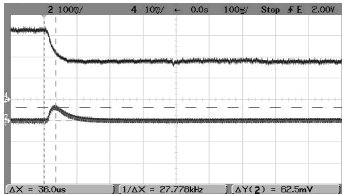
Step Load Transient Response (Vin=5V, Vout=2.5V, Cload=0, Iout=3A to 1.5A) Trace 2=Vout, 100 mV/div. Trace 4=Iout, 1A/div.
