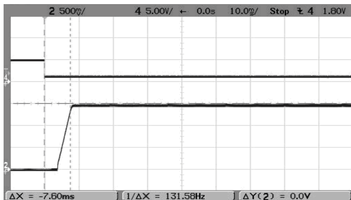
On/Off Enable Startup (Vin=5.5V, Vout=1.5V, Iout=3A, Cload=0)
