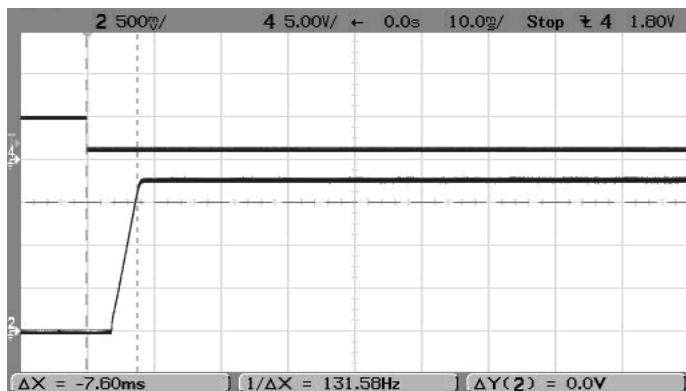
On/Off Enable Startup (Vin=5.5V, Vout=1.8V, Iout=3A, Cload=0) Trace 4=Enable, Trace 2=Vout
