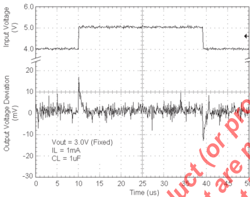
Fig. 36: Line Transient Response
