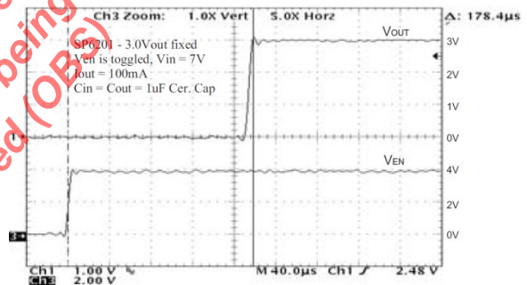
Fig. 25: Turn on time, I_o=100mA , 7V_{IN}
