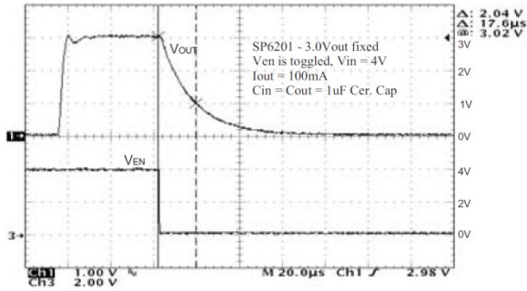
Fig. 28: Turn off time, I_o=100mA , 4V_{IN}
