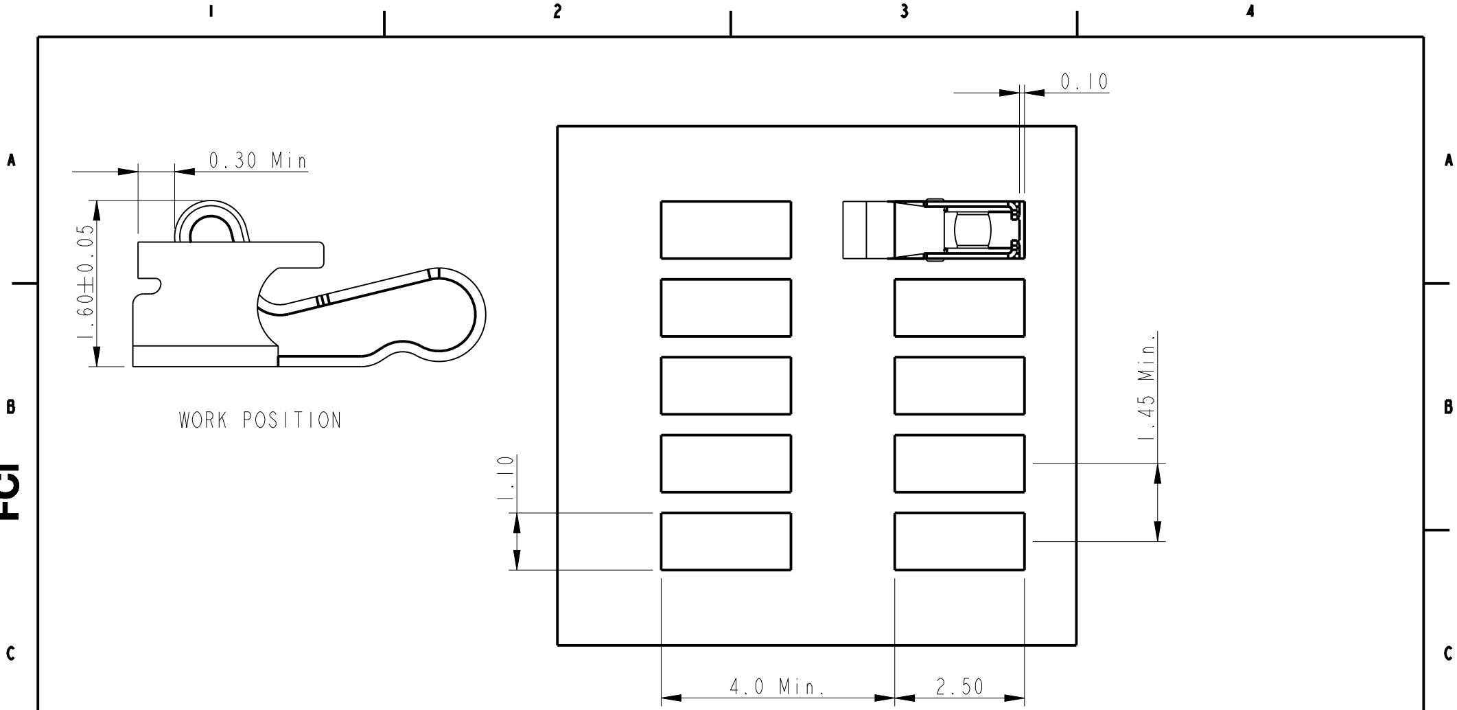
RECOMMENDED PCB DIMENSION & MIN PITCH TOLERANCE: +/-0.05mm
