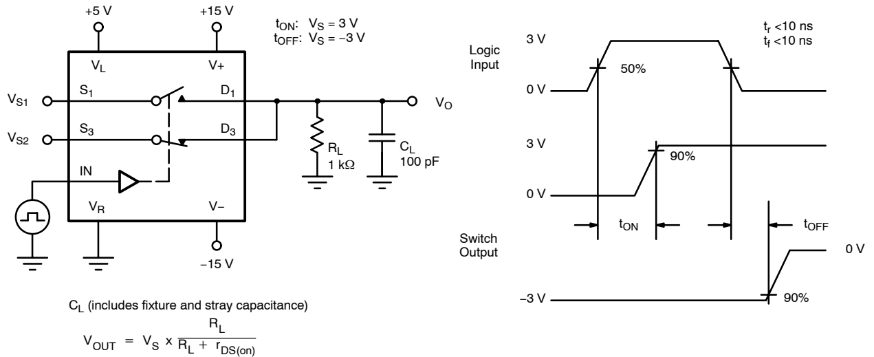
FIGURE 2. Switching Time
