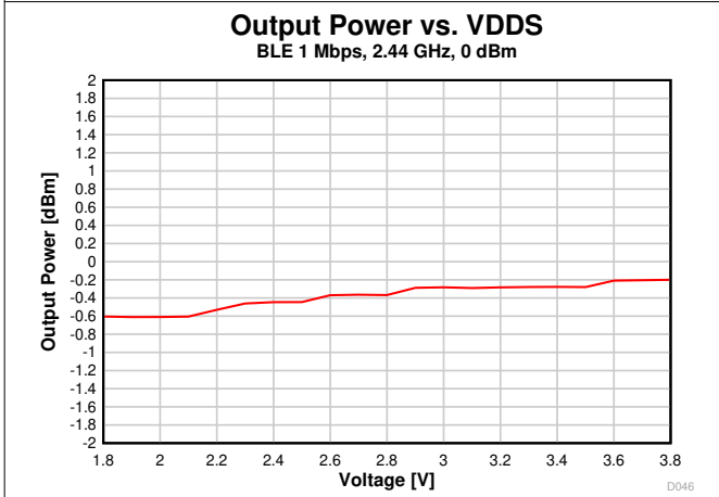
Figure 8-19. Output Power vs. Supply Voltage (VDD) (BLE 1 Mbps, 2.44 GHz)
