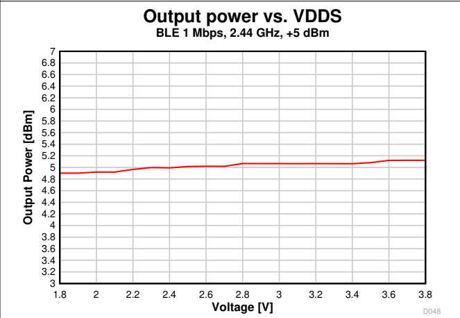
Figure 8-20. Output Power vs. Supply Voltage (VDD) (BLE 1 Mbps, 2.44 GHz, +5 dBm)
