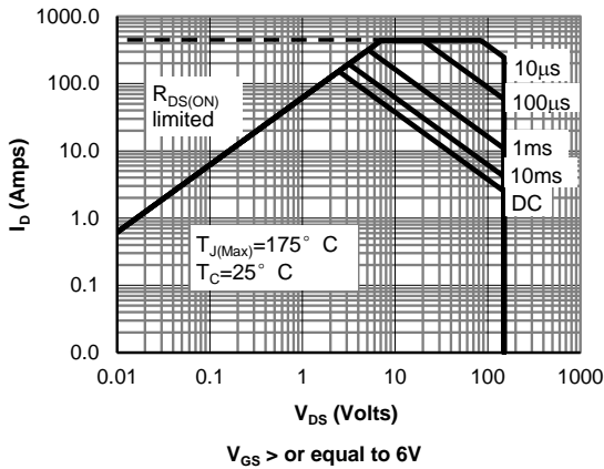
Figure 9: Maximum Forward Biased
