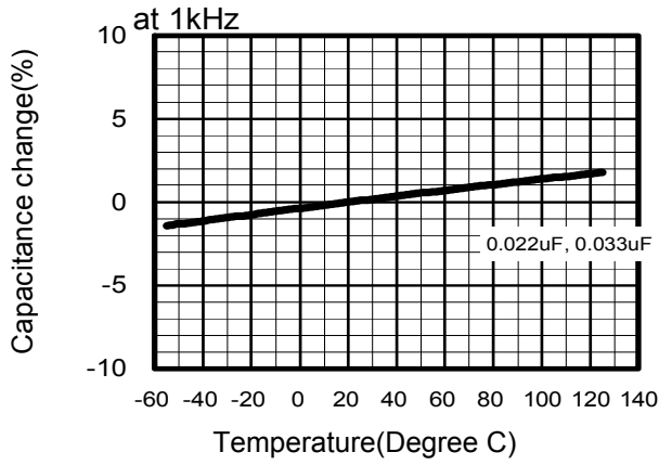
Temperature Characteristics
