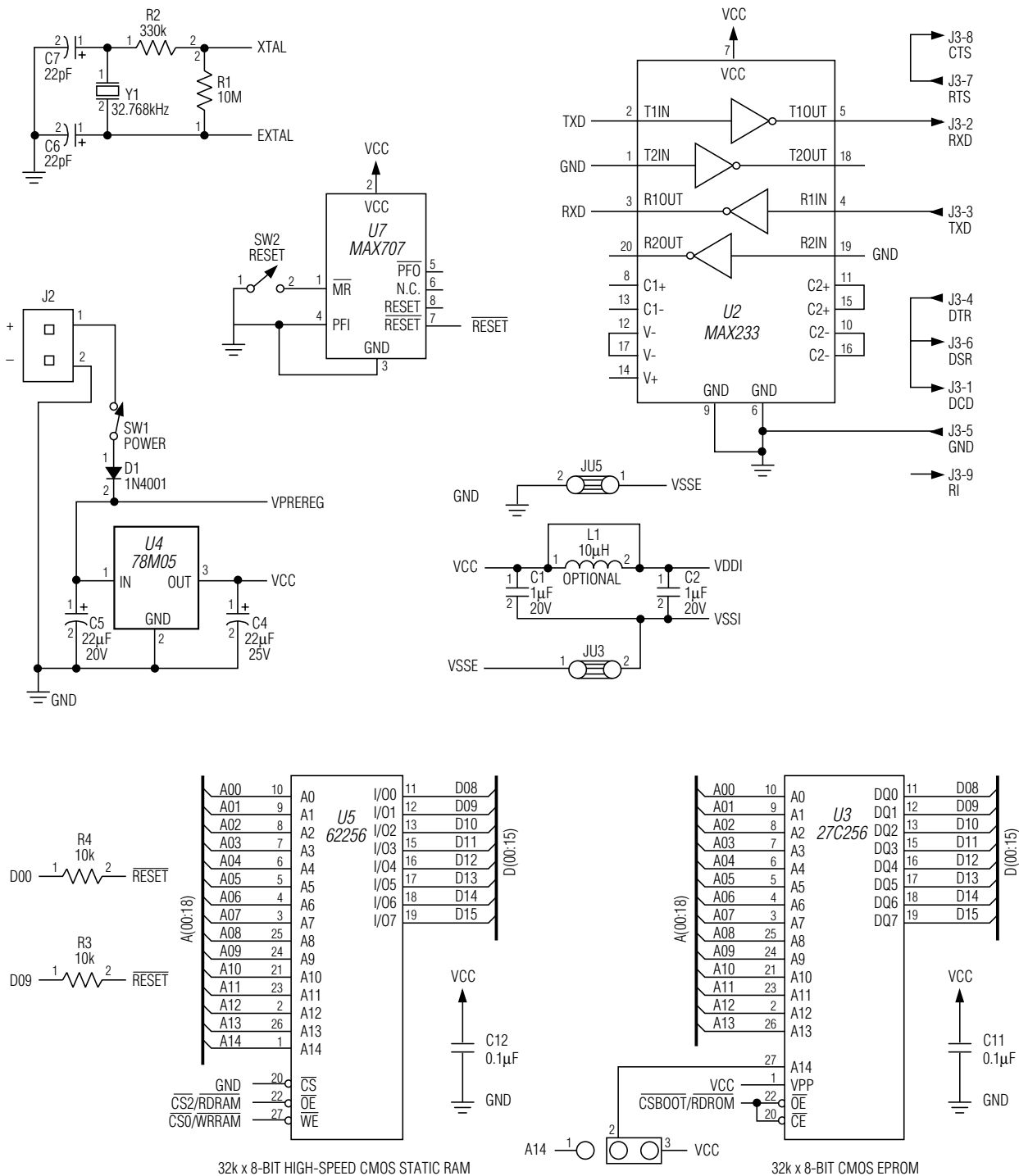
Figure 1. 68HC16 Module Schematic (continued)
