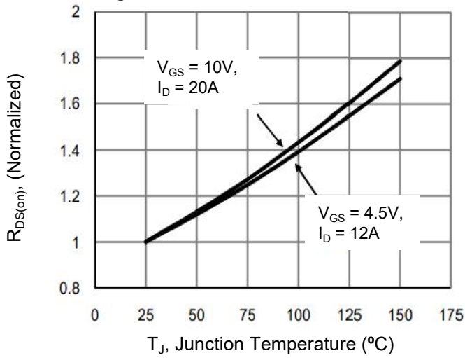
Figure 7. Drain-Source On-Resistance
