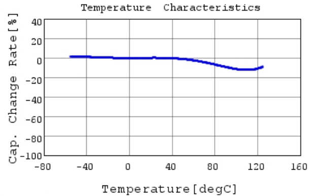
GRM31BR72J222KW01 C-Temp. capchange, DCOV, 1
