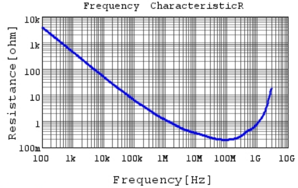
GRM31BR72J222KW01 R DCOV, 25degC
