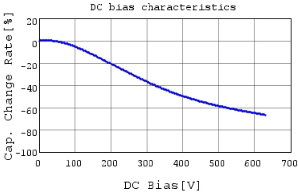
GRM31BR72J222KW01 C-DC bias capchange, 25.0c
