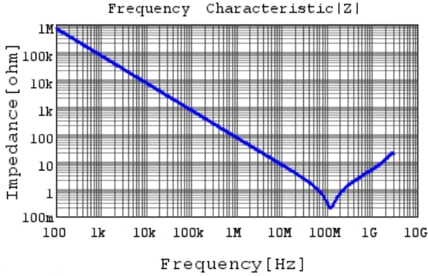
GRM31BR72J222KW01 |Z| DCOV, 25degC
