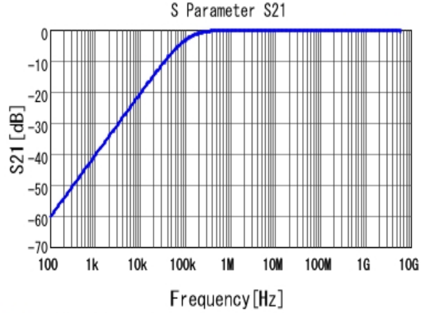
■ GCM188R71H153KA37 S21 DC0V, 25degC
