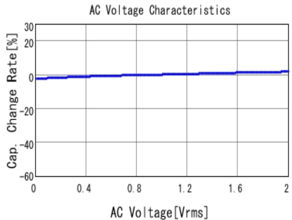
GCM188R71H153KA37 C-AC Voltage capchange, DCOV, 25.0d
