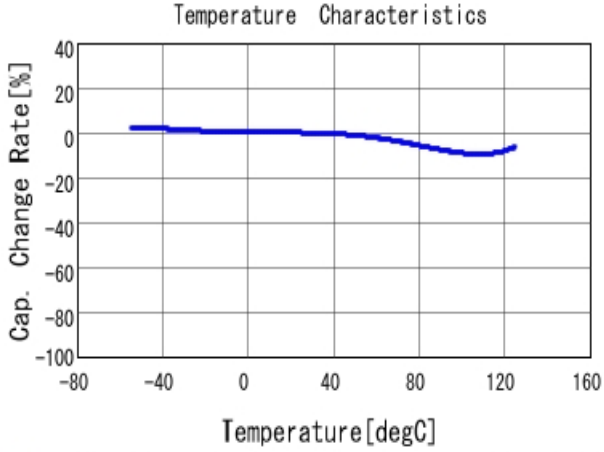
■ GCM188R71H153KA37 C-Temp. capchange, DC0.0V, AC1.0V r m
