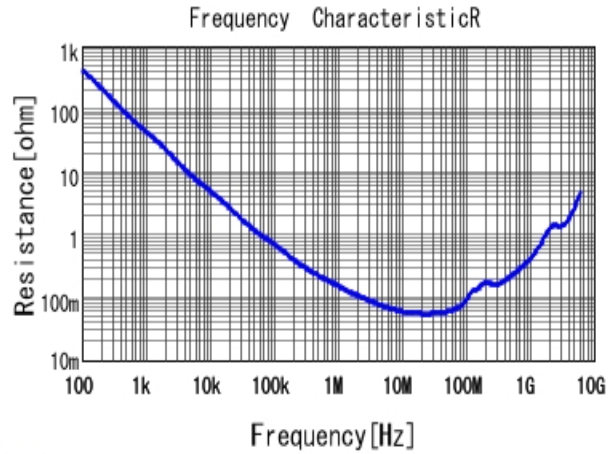
GCM188R71H153KA37 R DCOV, 25degC
