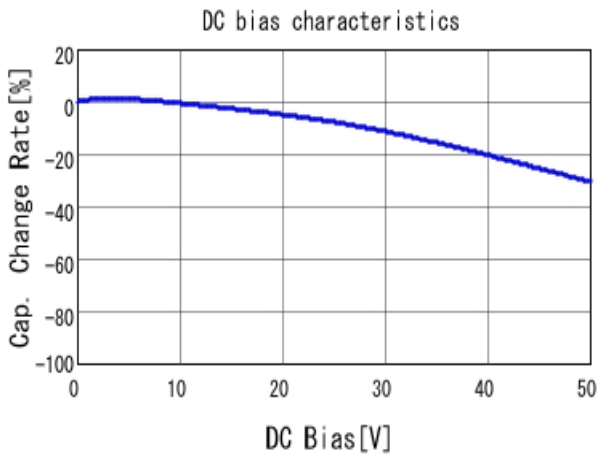
GCM188R71H153KA37 C-DC bias capchange, 25.0degC, AC1.
