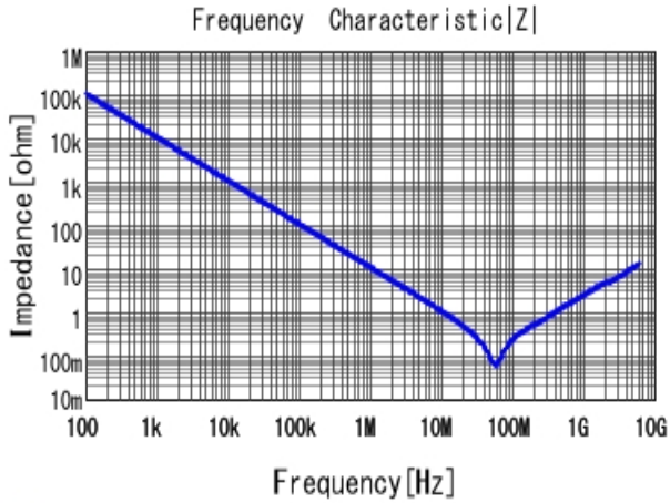
GCM188R71H153KA37 |Z| DCOV, 25degC
