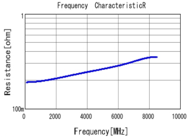
■ GJM1555C1H2R0WB01 R DCOV, 25degC
