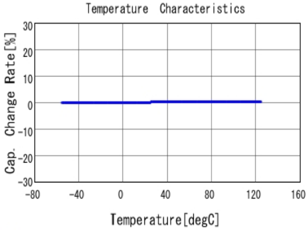
■ GJM1555C1H2R0WB01 C-Temp. capchange, DCOV, AC1Vrms
