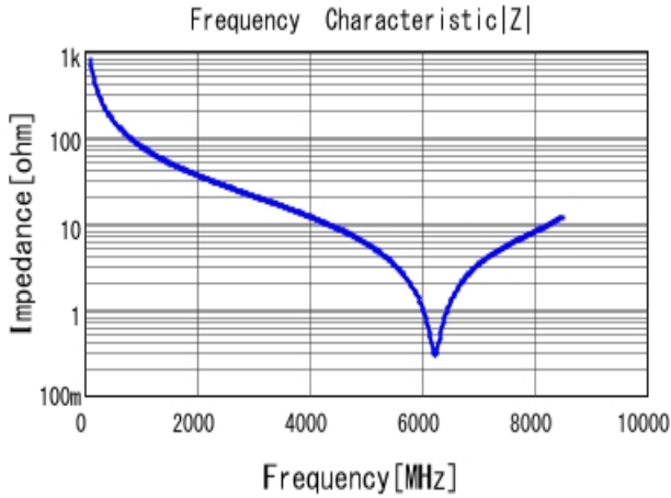
■ GJM1555C1H2R0WB01 |Z| DCOV, 25degC
