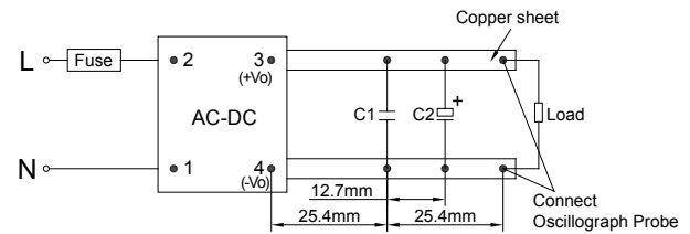
C1: Ceramic capacitor, 1µF; C2: Electrolytic capacitor, 10µF
