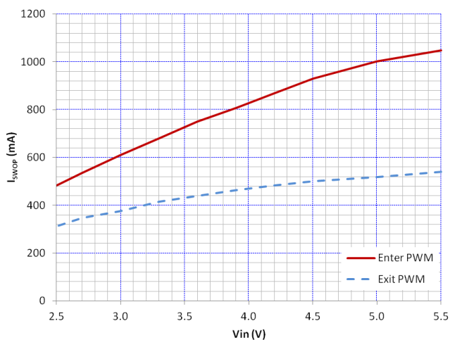
Figure 23. Switchover Point V_{OUT} = 1.50\text{ V}
