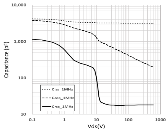
Figure 13. Capacitance Charge
