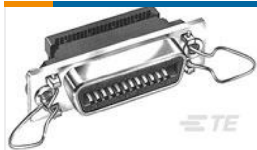
TE Part #5554434-1 EMI RCPT ASSY, 24 POSN, SHLD
