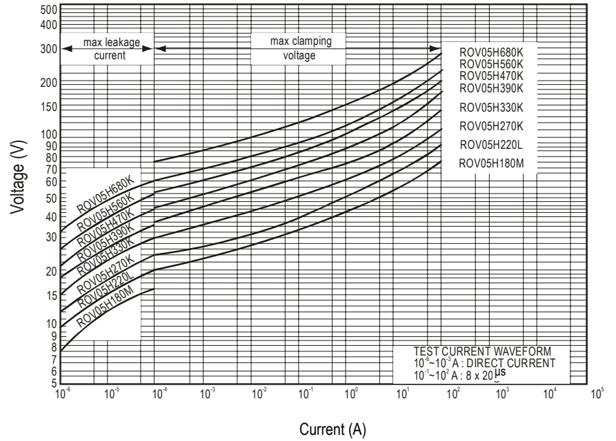
ROV05H180M – ROV05H680K
