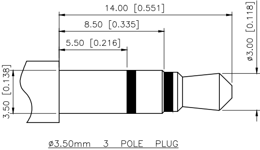
ø3.50mm 3 POLE PLUG
