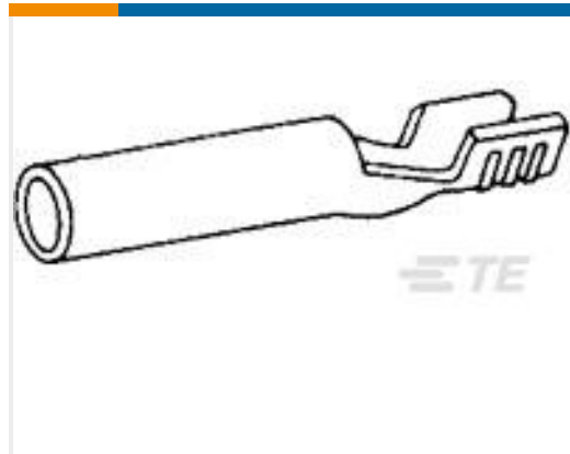
TE Part #63381-1 PIN .125 TERMINAL REC 22-18 AWG BR
