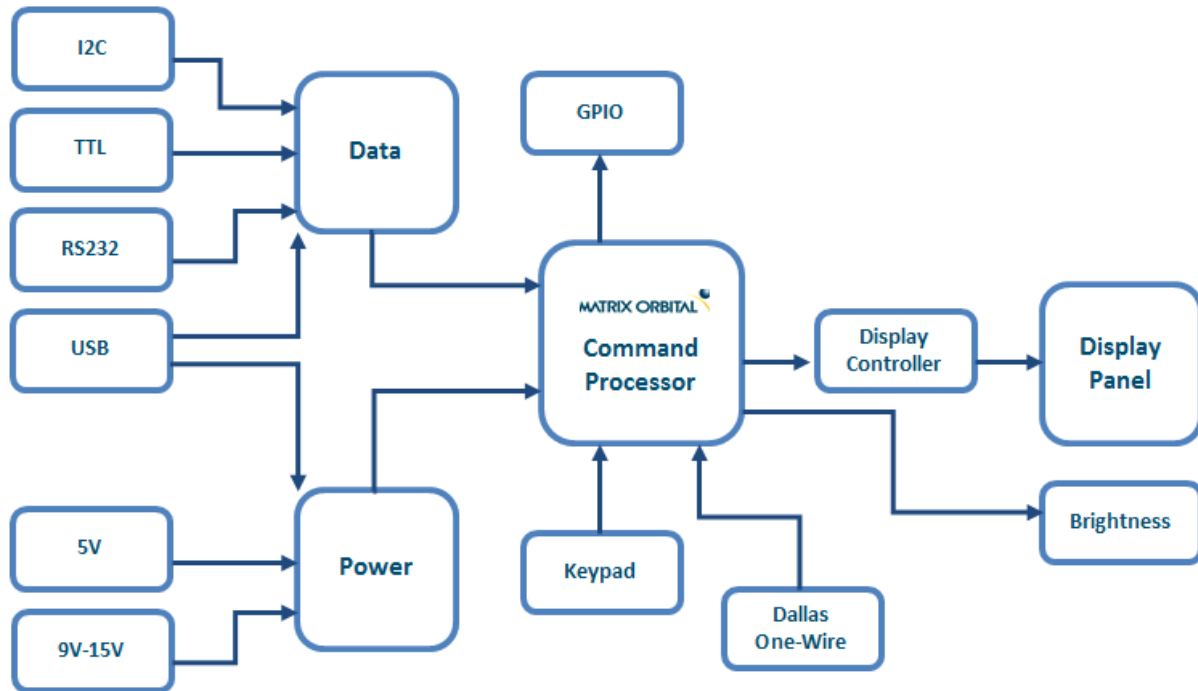
Figure 17: Functional Diagram
