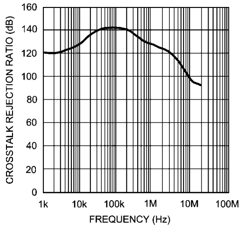
Crosstalk Rejection Ratio (LMP7712)
