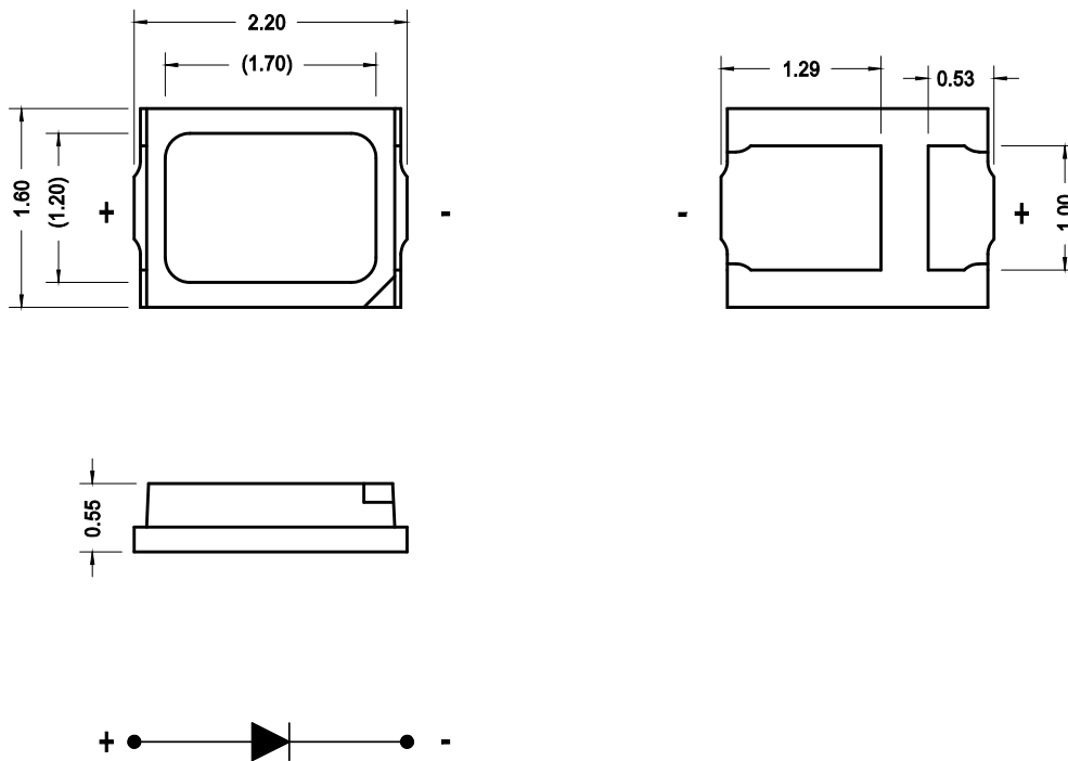
Figure 1: Package Drawing
