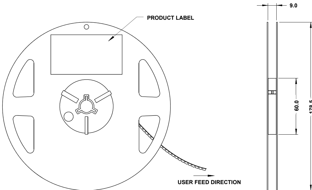
Figure 20: Reel Dimensions
