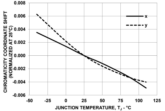
Figure 15: Chromaticity Coordinate Shift vs. Junction Temperature (6500K)
