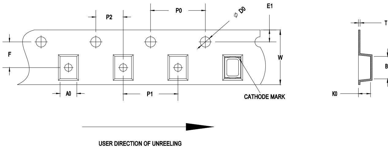
Figure 19: Carrier Tape Dimensions
