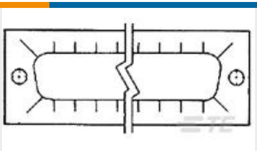
TE Part #5747025-3 RFI GASKET, SIZE 2, PLATED
