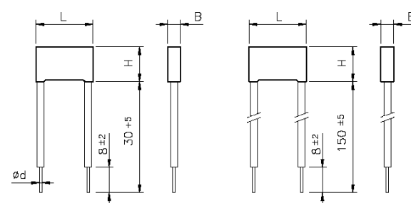
Insulated rigid leads
