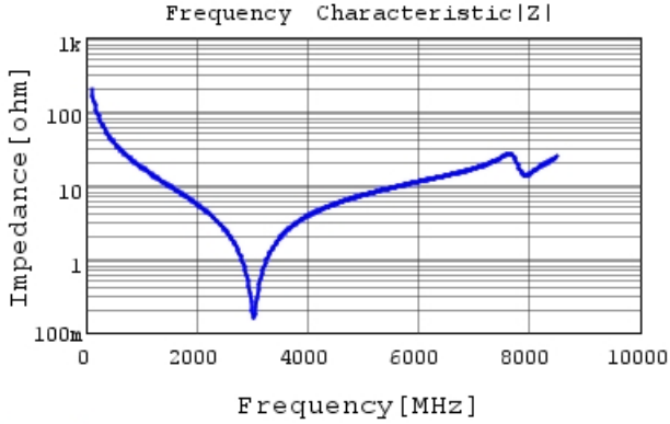
GJM1555C1H8R2CB01 |Z| DCOV, 25degC
