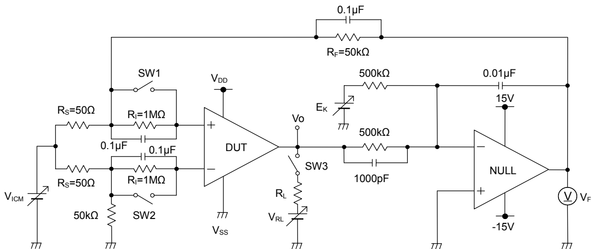
Figure 73. Test Circuit 1
