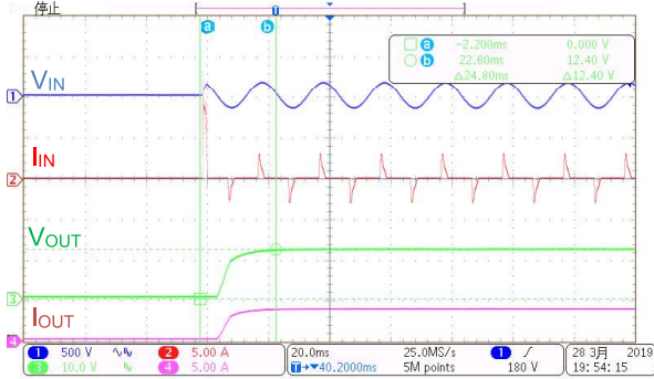
Figure 37. V_{IN} = 115 \text{ Vac} , I_{OUT} = 4.0 \text{ A}
