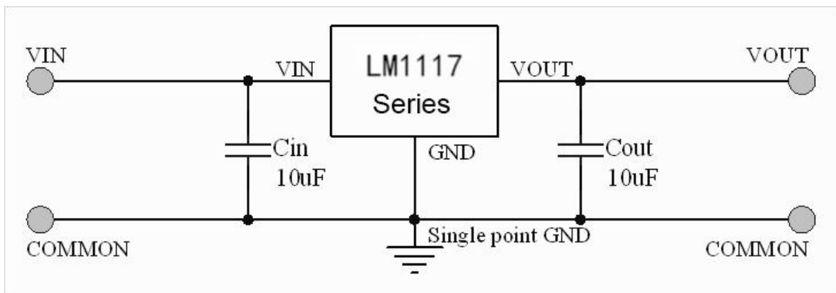
Application circuit of LM1117X fixed version
