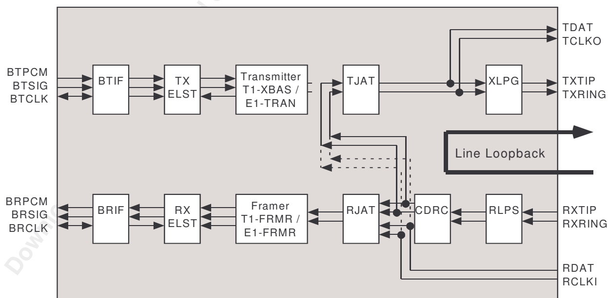
Figure 39 - Line Loopback
