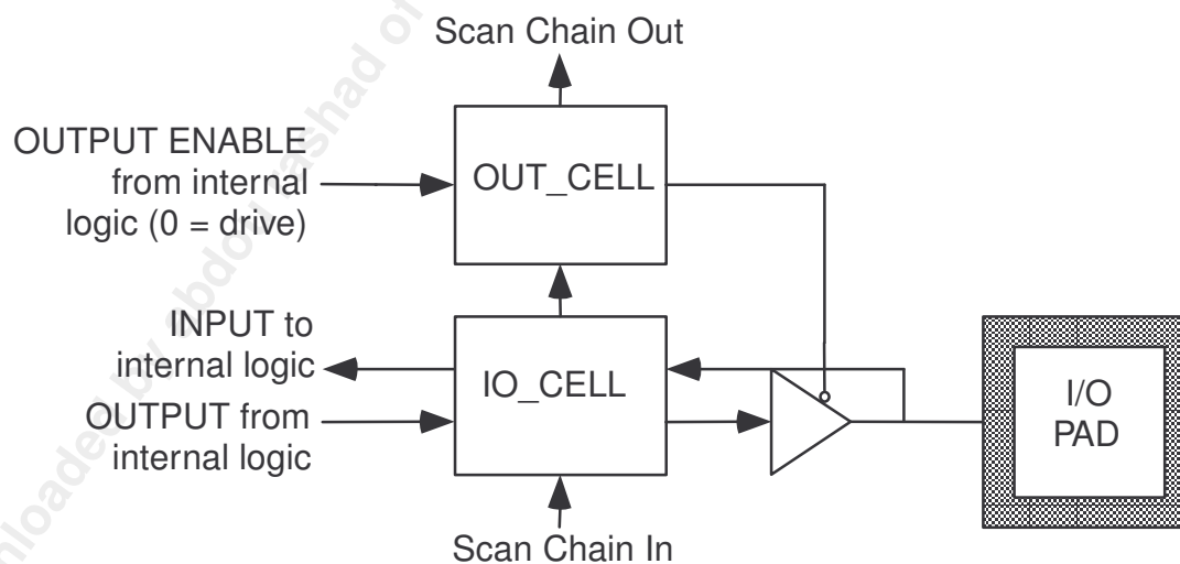
Figure 54 - Layout of Output Enable and Bidirectional Cells
