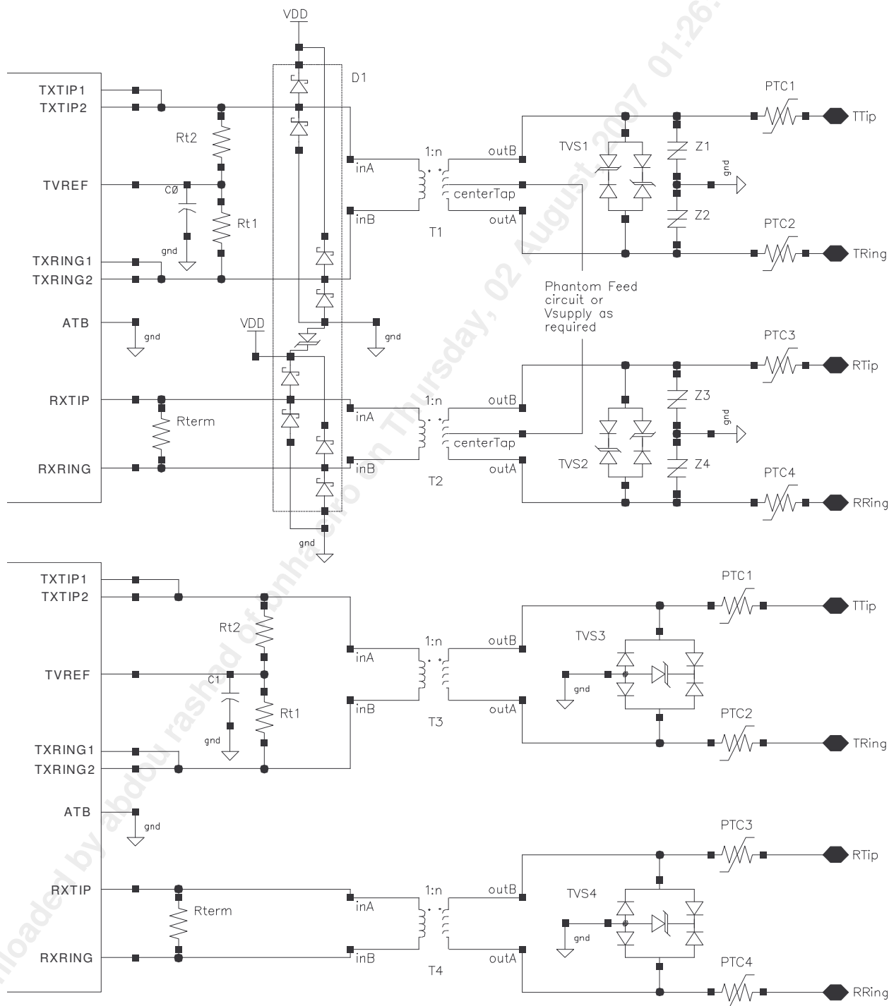
Figure 5 - External Analog Interface Circuits
