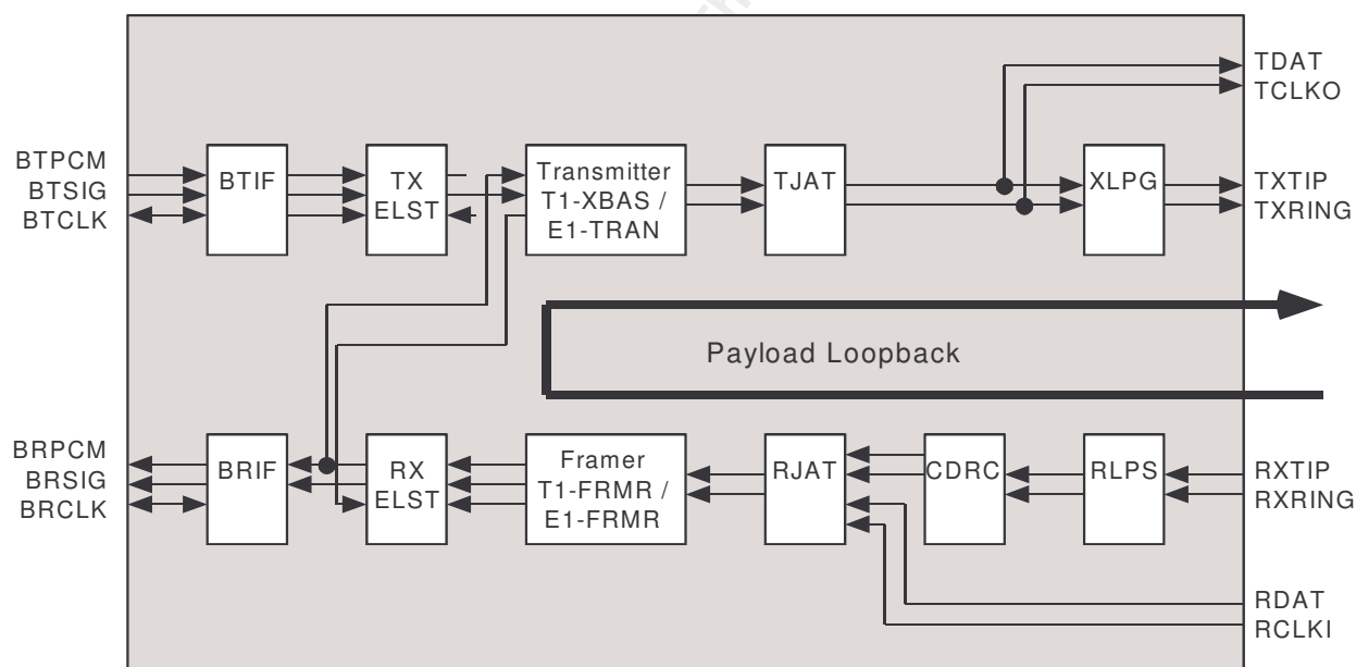
Figure 40 - Payload Loopback
