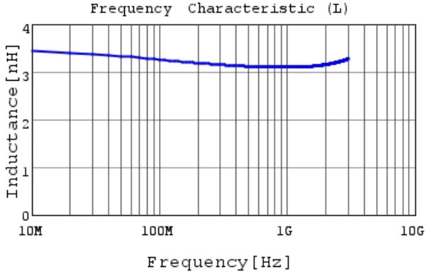
LQP03TN3N1B02 L
