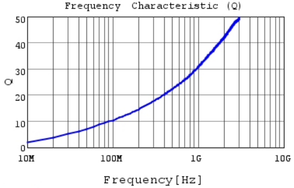
LQP03TN3N1B02 Q
