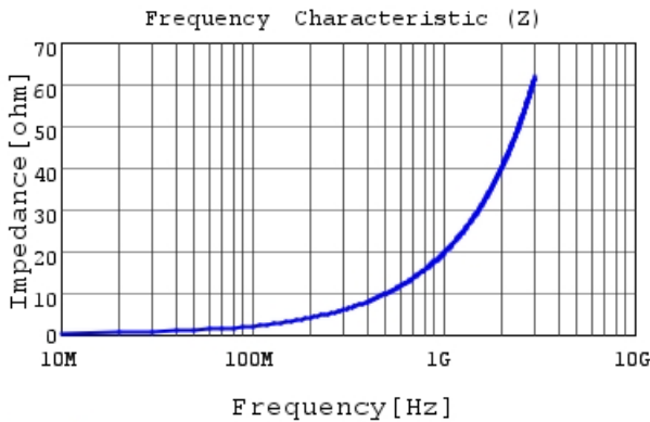
LQP03TN3N1B02 |Z|
