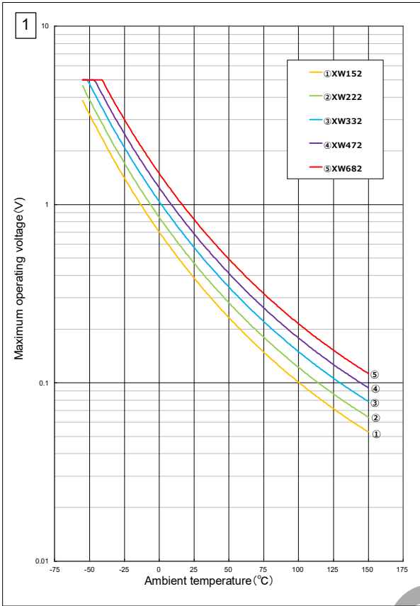
Graph of Maximum Operating Voltage Reduction Characteristics
