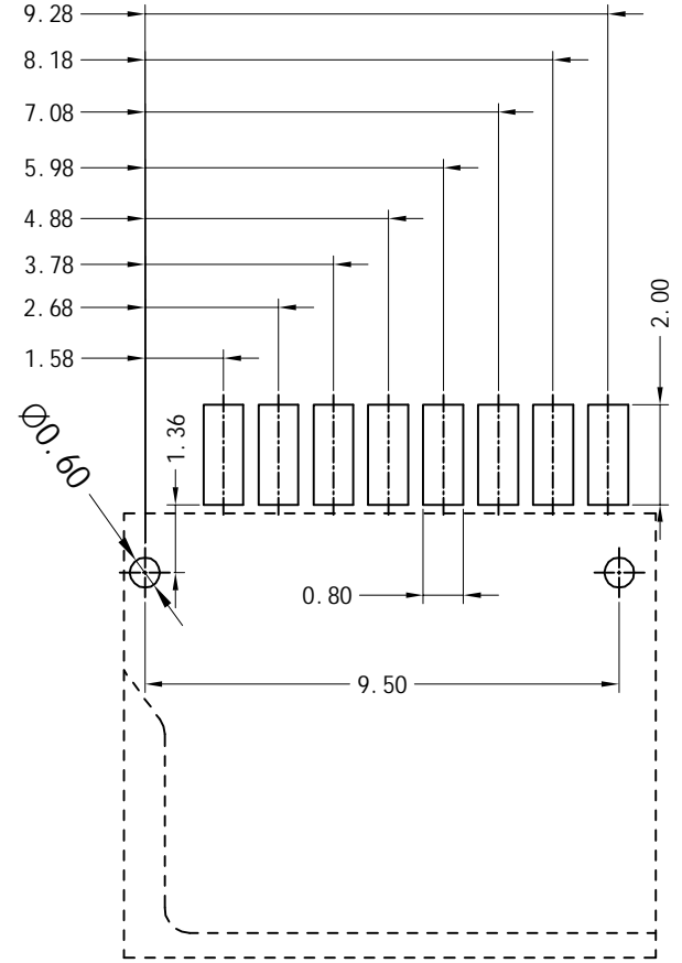
P. C. B LAYOUT
