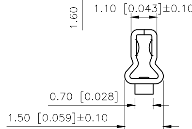
SECTION:C-C SCALE:1:1
