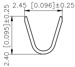
SECTION:A-A SCALE:1:1
