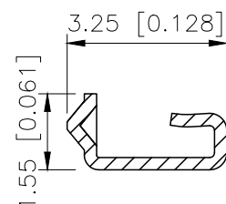
SECTION:B-B SCALE:1:1
