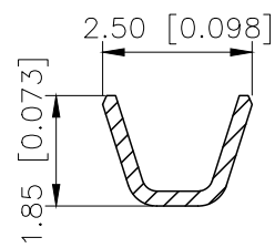
SECTION:A-A SCALE:1:1
