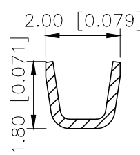
SECTION:C-C SCALE:1:1
