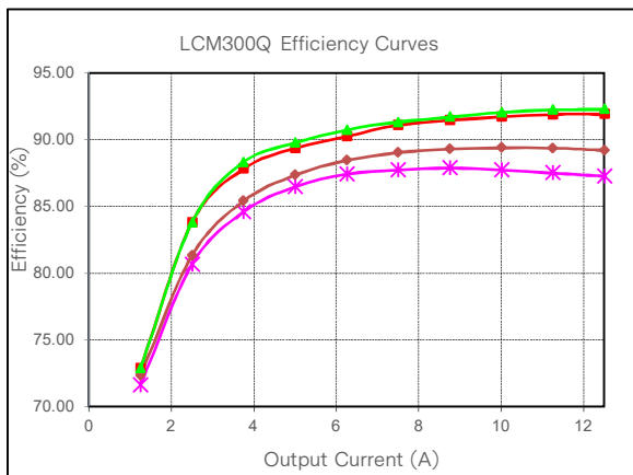
Figure 31: LCM300Q Efficiency Curve @ 25°C Loading: I_{O\_main} = 10\%I_{O\_max} increment to 12.5A, I_{SB} = 0A (5V)
