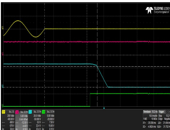
Figure 36: LCM300U Hold-up Time Vin = 90Vac / 47Hz / 0° Load: Io = 8.4A (36V), I SB = 2A (5V) Ch 1: AC Mains Ch 2: V SB Ch 3: Vo Ch 4: G_DCOK_C
