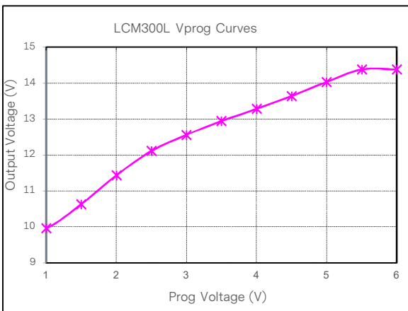
Figure 11: LCM300L Output Voltage Adjustment by Vprog @ 25°C - 115Vac (magenta x) Loading: I_O = 0A (12V), I_{SB} = 0A (5V)
