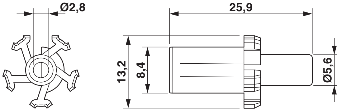
Dimensional drawing
