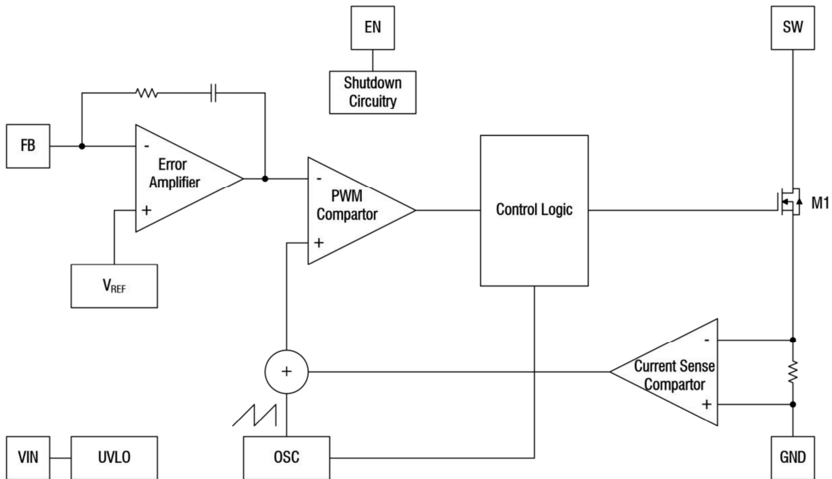
Figure 2. SDB628 Block Diagram
