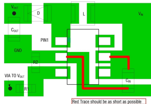
Figure 3. SDB628 Suggested Layout
